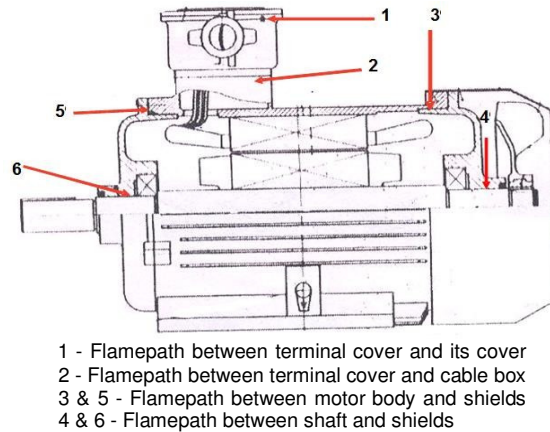
Figure 1. Flamepath locations in Exd motor
